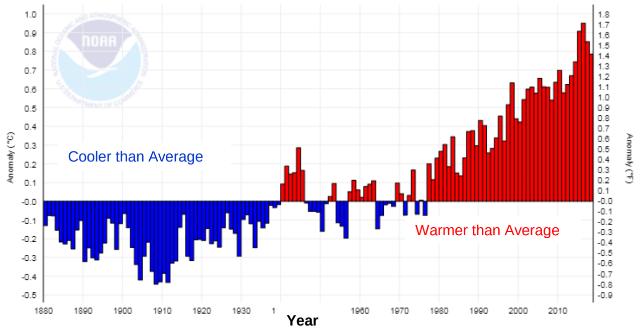
Figure 1. Global land and air temperature anomalies. Normalization period includes 1981-2010. Source: NOAA: https://www.ncdc.noaa.gov/cag/global/time-series/globe/land_ocean/yttd/12/1880-2019 ).
