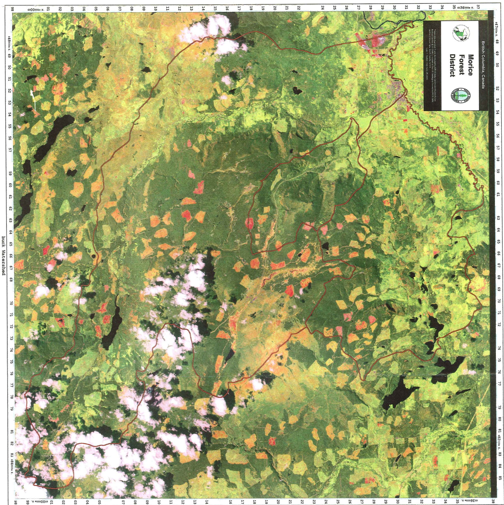
Figure 3. 2000 Landsat 7 Image of the Buck Watershed.
