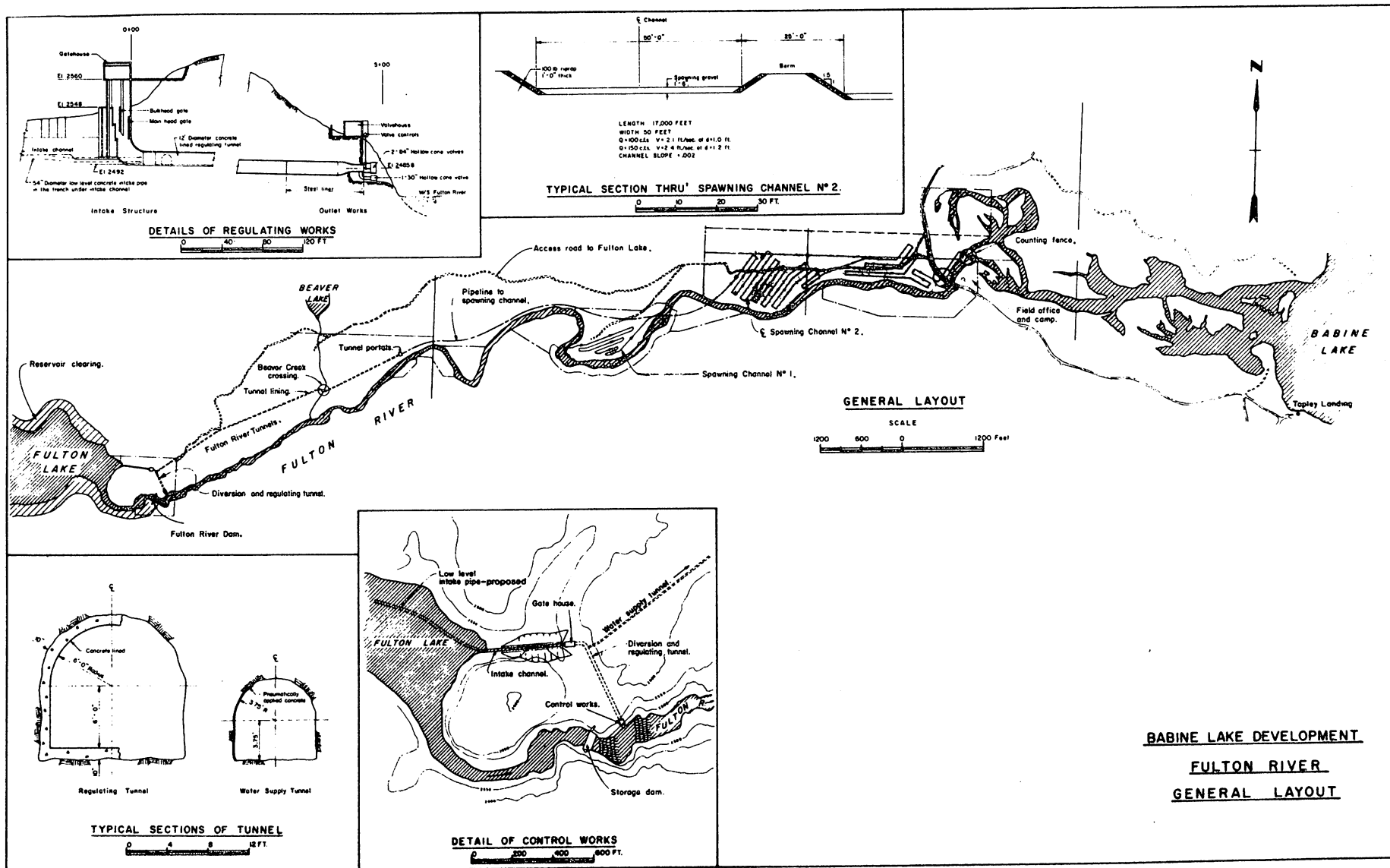
Figure 3: Schematic layout of the Fulton River enhancement project including a profile of the water regulatory works.
